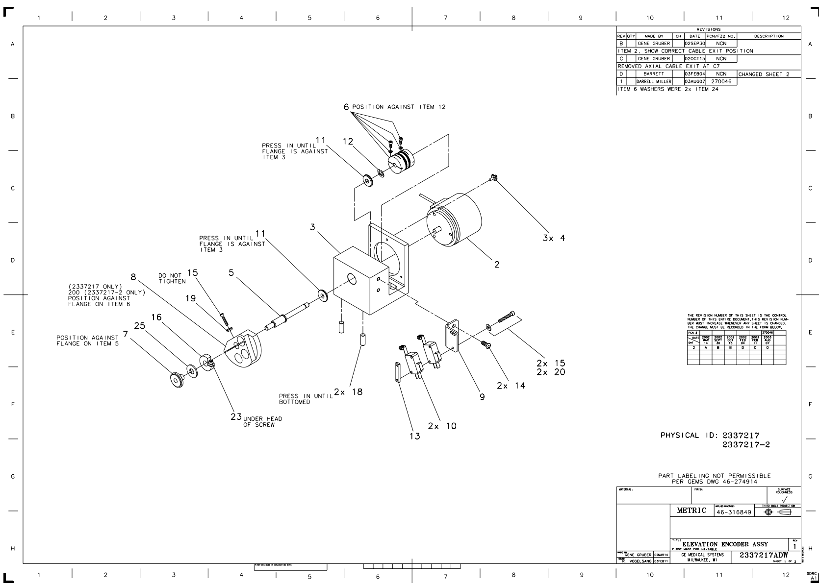
Figure 2-15 Encoder Assembly, Elevation - H Power (2337217, sheet 1, rev 1)
