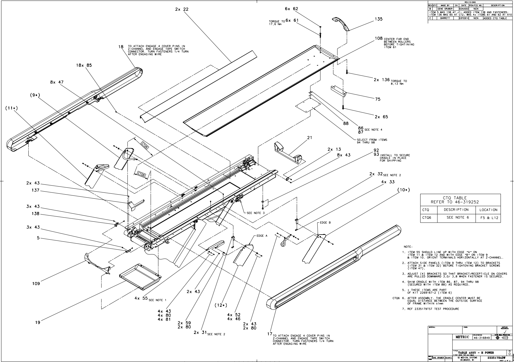
Figure 2-2 Table Assembly - H Power (2335179, sheet 2, rev 0)
