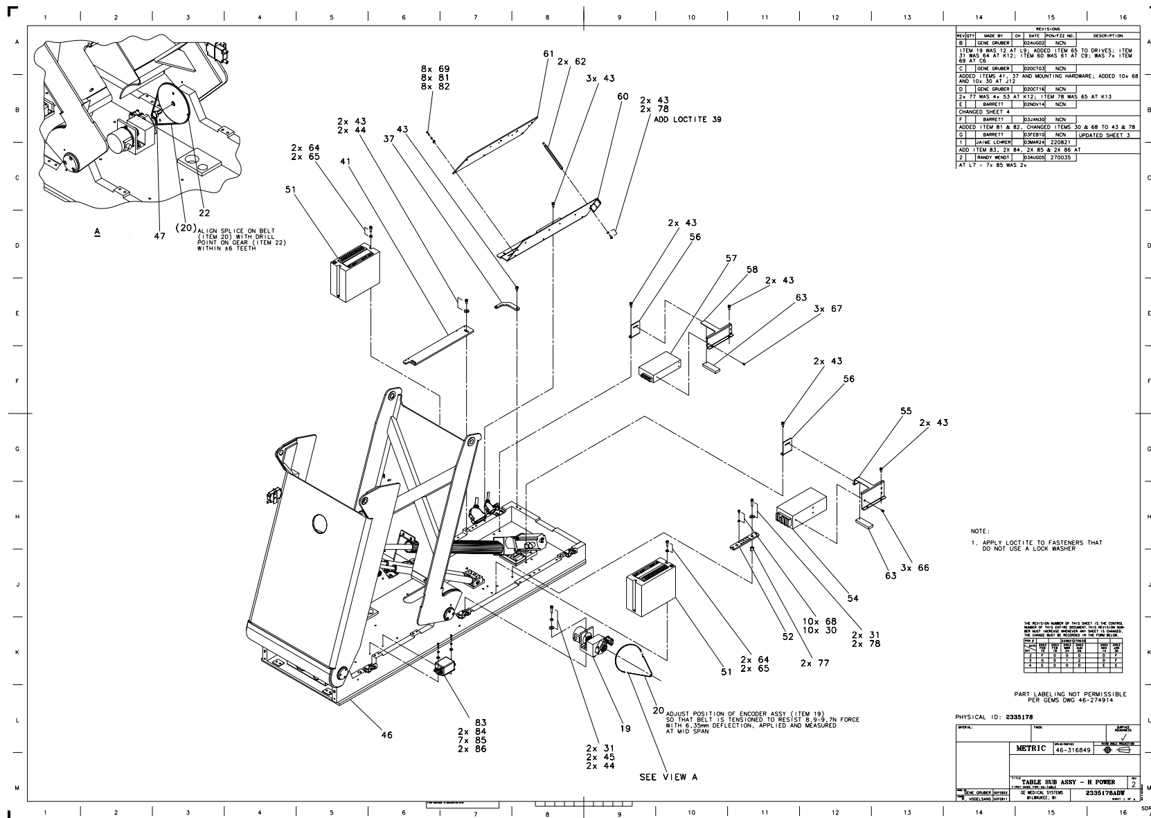
Figure 2-6 Table Subassembly (2335178, sheet 1, rev 2)
