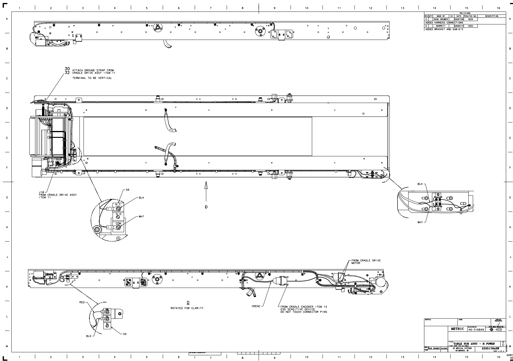
Figure 2-9 Table Subassembly (2335178, sheet 4, rev 0)
